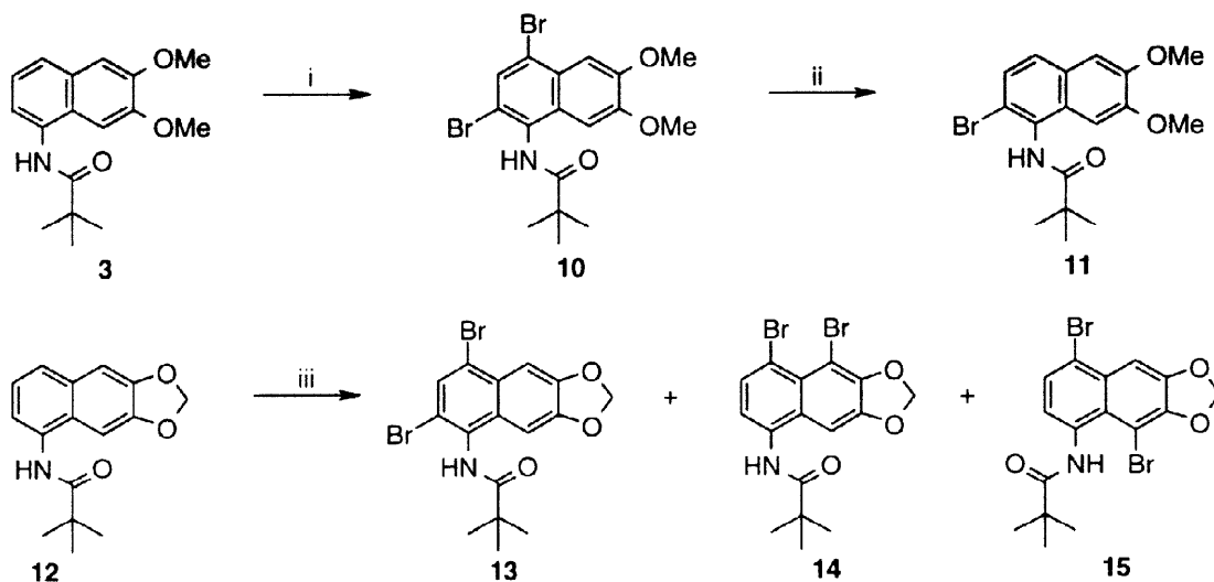
Scheme 3 Reagents and conditions: i) \text{Br}_2 , NaOAc, AcOH, THF, 45 – 50^\circ\text{C} , 6 h, 70%; ii) 2.0 eq. tBuLi, THF, TMEDA, -78^\circ\text{C} , 1 h, then AcOH, -78 to 0^\circ\text{C} , 15 min, 48%; iii) \text{Br}_2 , NaOAc, AcOH, 45 – 50^\circ\text{C} , 2 h, 13 25%, 14 + 15 34%.
