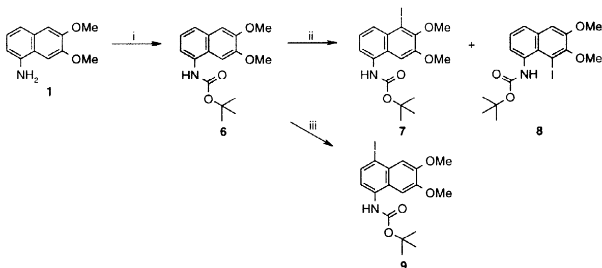
Scheme 2 Reagents and conditions: i) (\text{Me}_3\text{CCO}_2)_2\text{O} , THF, \Delta , 2 h, 85%; ii) 2.8 eq. tBuLi, THF, -40 to -20^\circ\text{C} , 5 h, then \text{ICH}_2\text{CH}_2\text{I} , -78 to 25^\circ\text{C} , 18 h, 30%; iii) 2.8 eq. tBuLi, \text{Et}_2\text{O} , DME, -40 to -20^\circ\text{C} , 5 h, then \text{ICH}_2\text{CH}_2\text{I} , -78 to 25^\circ\text{C} , 18 h, 22%.
