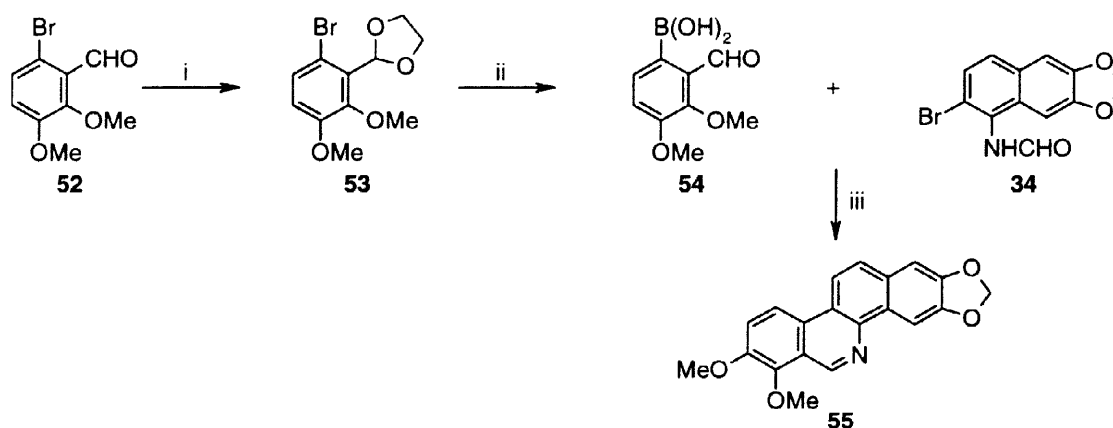
Scheme 8 Reagents and conditions: i) HOCH 2 CH 2 OH, p-TSA, toluene, Δ, 89%; ii) nBuLi, THF, -78°C, then B(O i Pr) 3 , -78 to 25°C, then dil. HCl, Δ, 60%; iii) Pd(PPh 3 ) 4 , DME, aq. NaHCO 3 , 3h, Δ, then dil. HCl, Δ, 58%.
