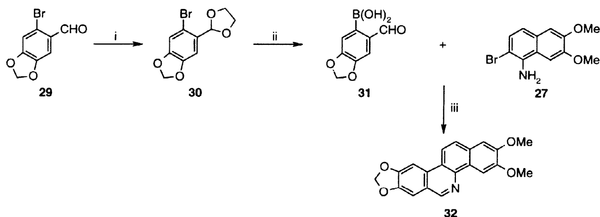
Scheme 5 Reagents and conditions: i) HOCH 2 CH 2 OH, p-TSA, toluene, Δ, 89%; ii) nBuLi, THF, -78°C, then B(O i Pr) 3 , -78 to 25°C, then dil. HCl, Δ, 61%; iii) Pd(OAc) 2 , PPh 3 , DME, aq. Na 2 CO 3 , 21 h, 35%.
