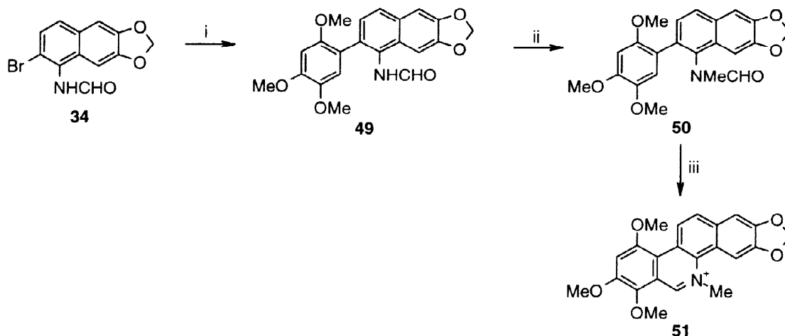
Scheme 7 Reagents and conditions: i) 48 , \text{Pd}(\text{OAc})_2 , \text{PPh}_3 , DME, aq. \text{Na}_2\text{CO}_3 , 1.25–4 h, 94%; ii) MeI, NaH, THF or DMF, 0 – 25^\circ\text{C} , 1.5 h, 96%; iii) \text{POCl}_3 , MeCN, reflux 3 h, 89%.
