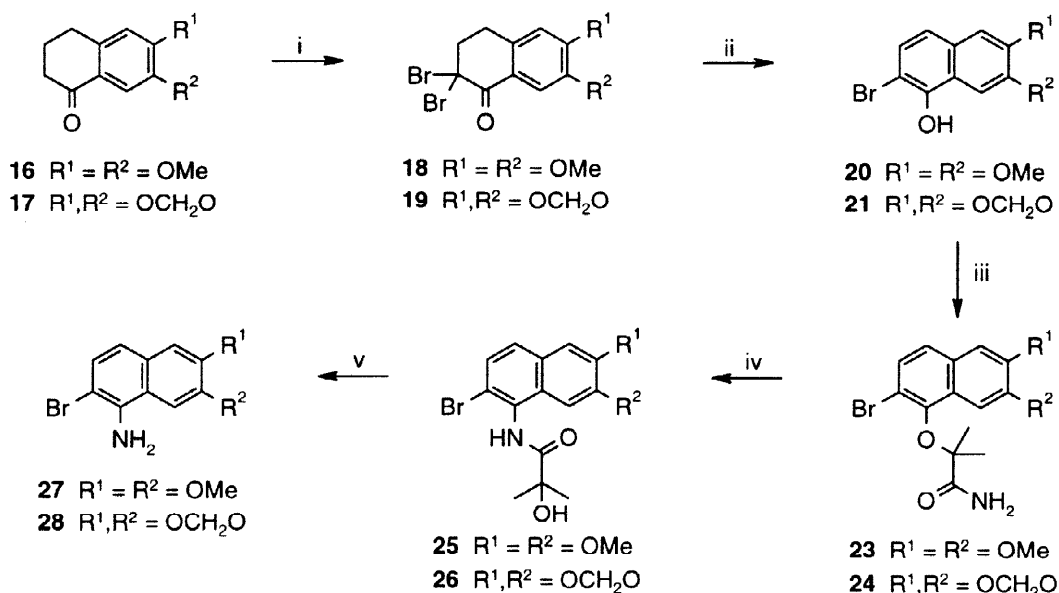
Scheme 4 Reagents and conditions: i) Br 2 , CHCl 3 , 25°C, 18 h, 18 66%, 19 97%; ii) DBU, MeCN, 40–45°C, 20 min, 20 93%, 21 97%; iii) 22 , granular NaOH, DMPU, 25°C, 2–5 h, 23 93%, 24 93%; iv) NaH, 4:1 DMF-DMPU, 100°C, 2 h, 25 93%, 26 96%; v) 80% aq. NaOH, MeOH, reflux, 2–4 d, 27 82%, 28 74%.
