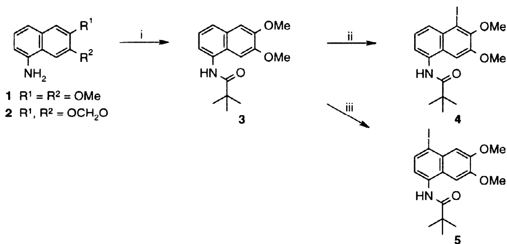
Scheme 1 Reagents and conditions: i) 1 , \text{Me}_3\text{CCOCl} , \text{Et}_3\text{N} , MDC, 0-5^\circ\text{C} , 1 h, 87%; ii) 3.0 eq. n\text{BuLi} , THF, -20 to 25^\circ\text{C} , 5 h, then \text{I}_2 , -78 to -12^\circ\text{C} , 16 h, 17%; iii) 3.0 eq. t\text{BuLi} , DME, -60 to 25^\circ\text{C} , 3 h, then \text{I}_2 , -78 to -12^\circ\text{C} , 16 h, 40%.
